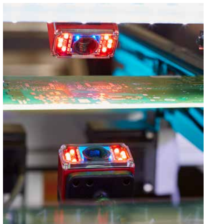
MicroHAWK cameras gather data from minuscule codes placed on a circuit board.
