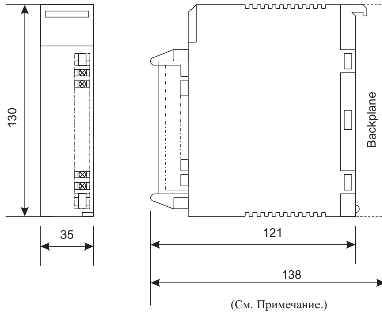
C200H-OA223
