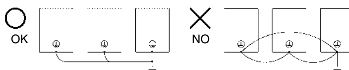
Fig 7 Ground Wiring
