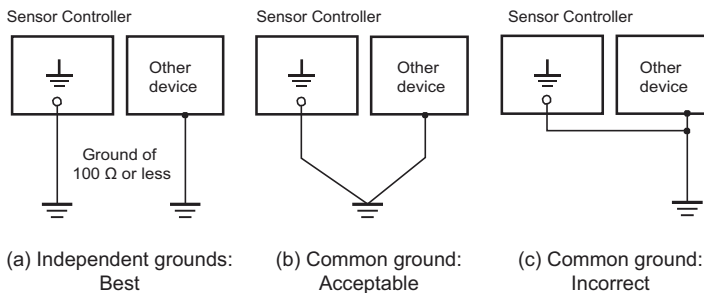
Grounding Methods
