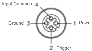
Connector T (Trigger) M12 4-pin Socket
