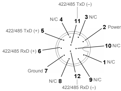
Connector P/M (All Models) M12 12-pin Plug
