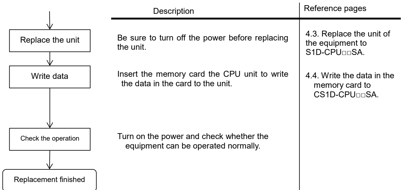
Figure 2-2: Replacement flow using a memory card
