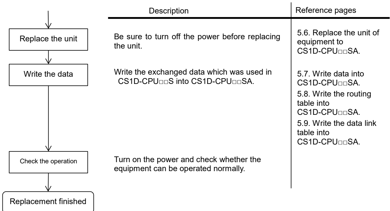
Figure 2-4: Replacement flow using the support tool
