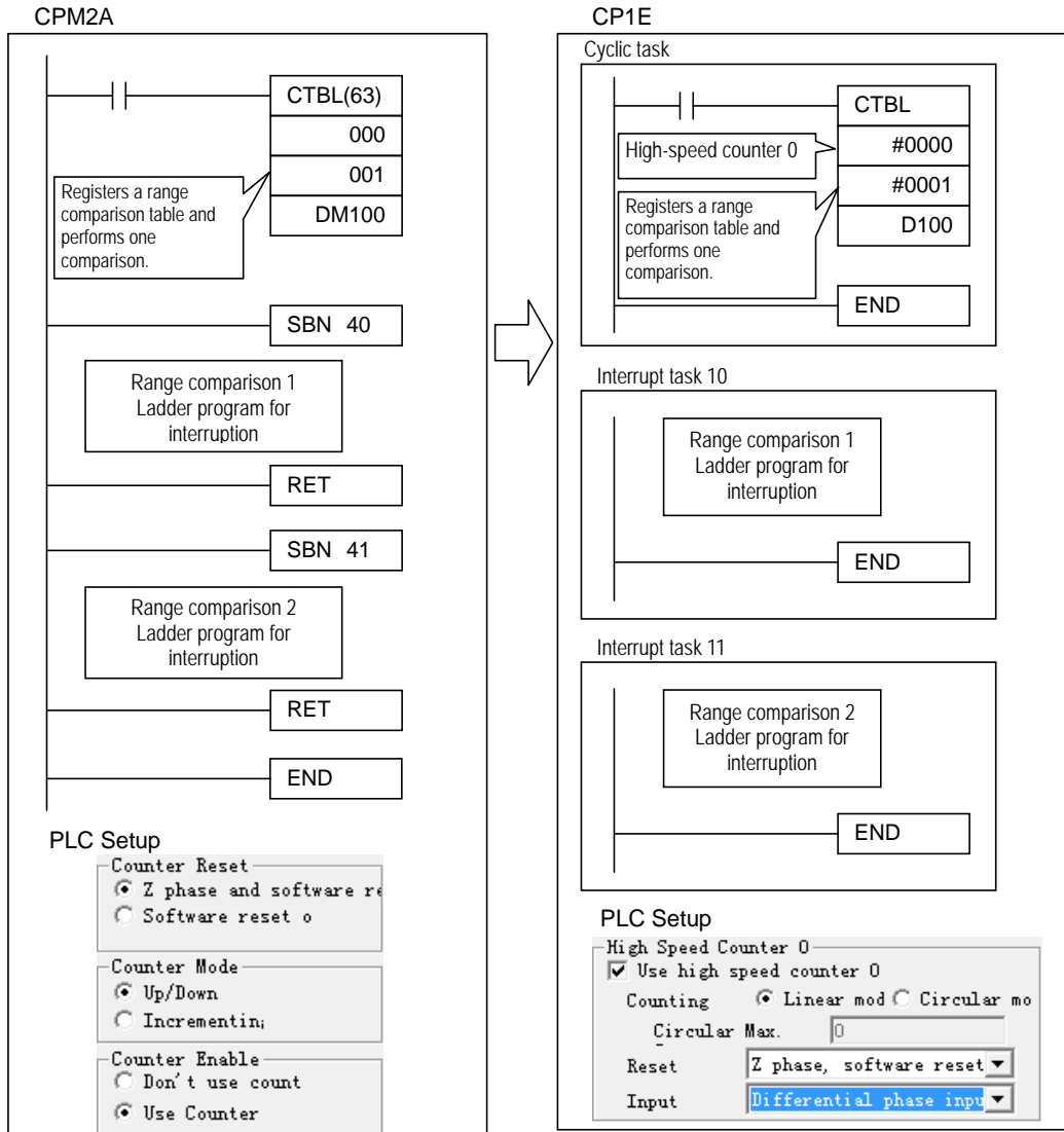
DM setting for CTBL instruction
