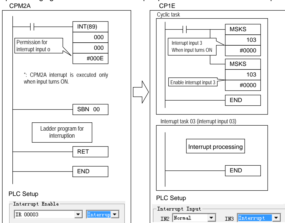
Example: Changing the CPM2A "0.03: Interrupt input 0" to the CP1E "0.03: Interrupt input 3"
