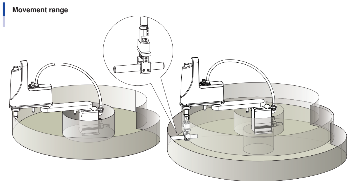
Figure A: Movement range of robot itself
