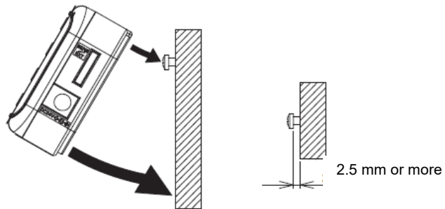
Enlarged Hook Screw Section View
