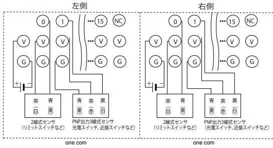
DRT2-OD32SL
