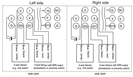
DRT2-ID32SLH-1
