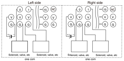
DRT2-MD32SLH
