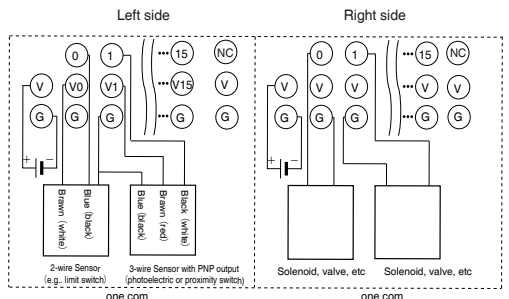
DRT2-MD32SLH-1
