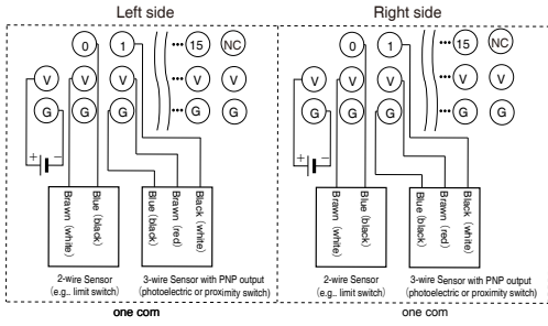
DRT2-OD32SL
