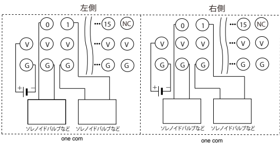
DRT2-MD32SL
