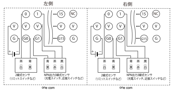
DRT2-ID32SLH-1
