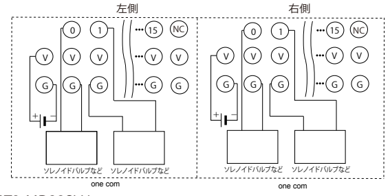
DRT2-MD32SLH
