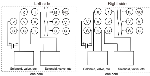
DRT2-MD32SL
