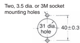
Mounting Holes
