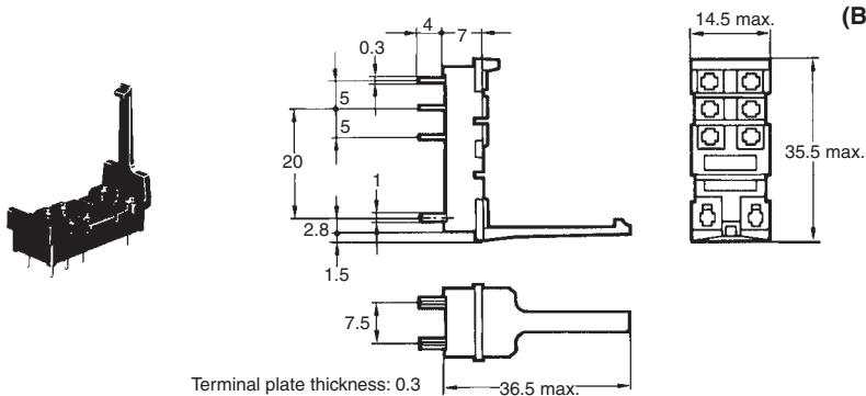
P2R-05A (1-pole)
