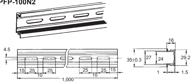
PFP-100N2
