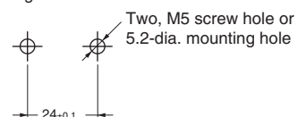
Mounting Hole Dimensions
