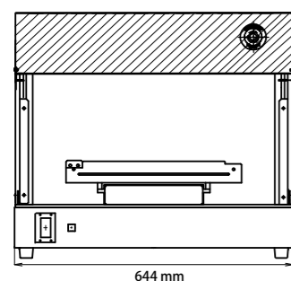
Exterior dimension (Front view)
