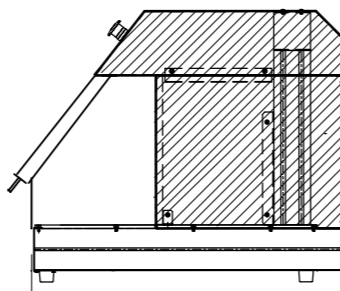
Area sensor attached type(Side view)
