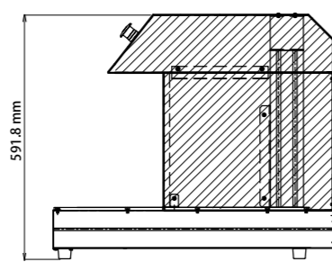
Standard type(Side view)
